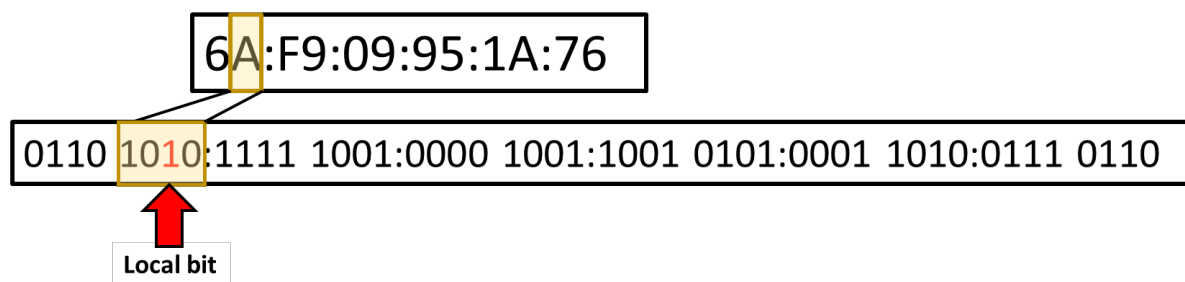
Figure 4 – Local Bit Within MAC Address
